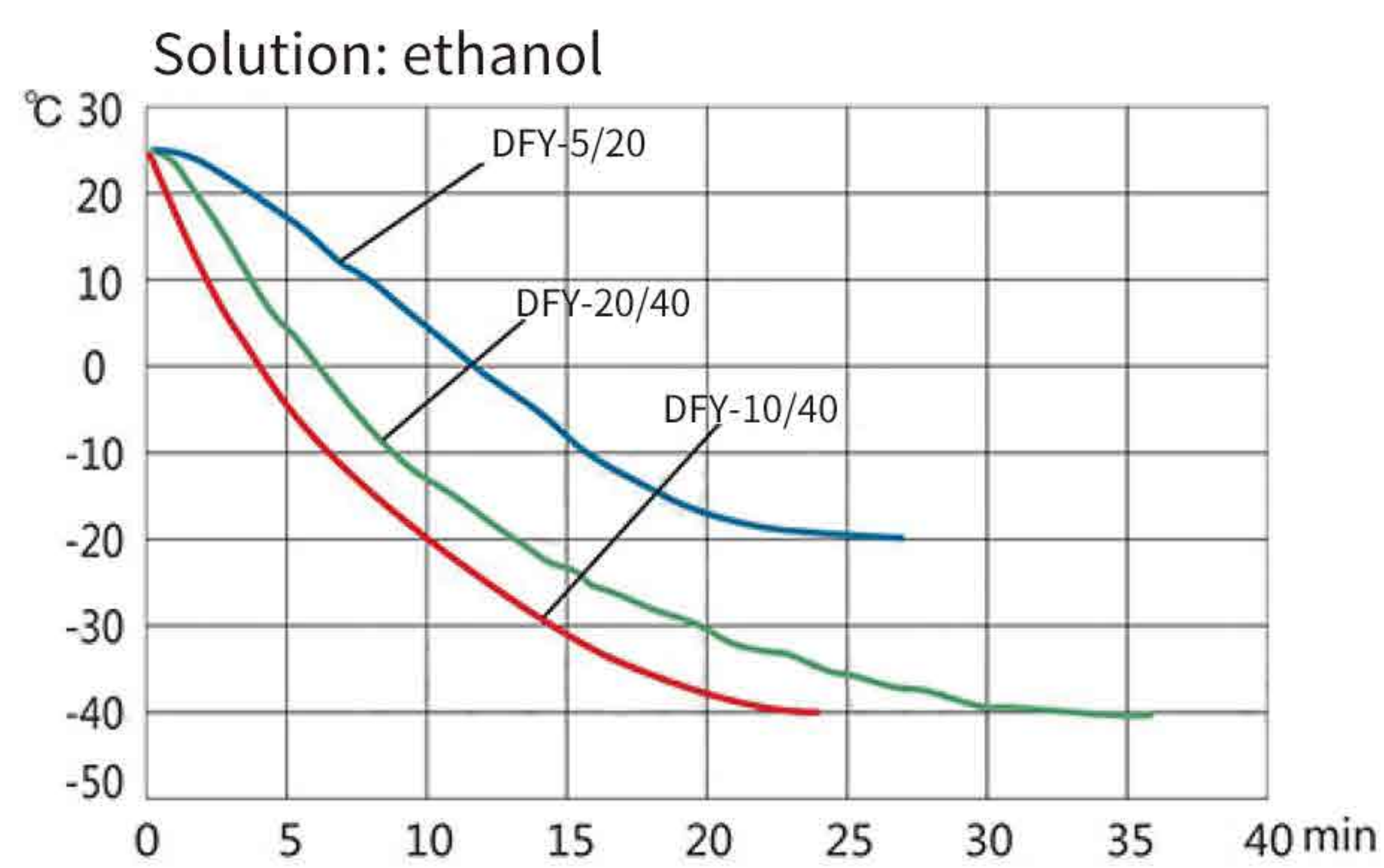
DFY-5/20, DFY-10/40, DFY-20/40 cooling curve
