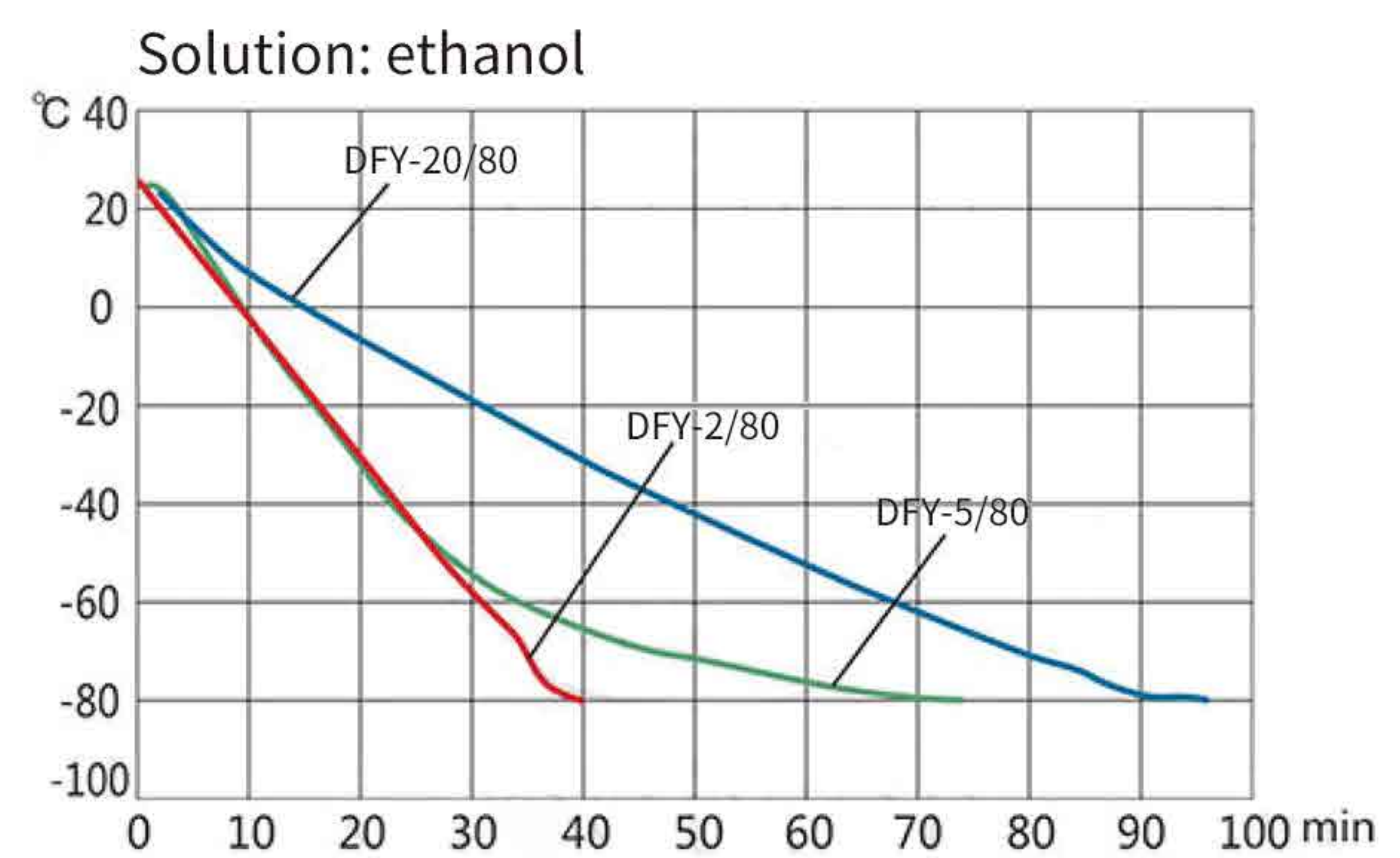
DFY-20/80, DFY-5/80, DFY-2/80 cooling curve
